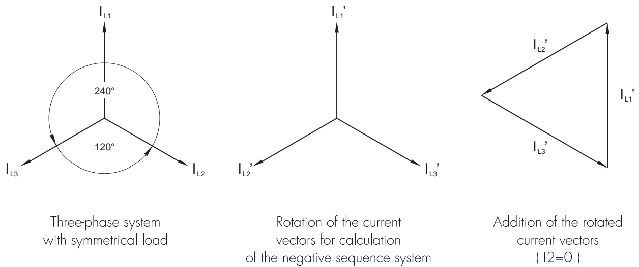
Fig. 4.1: Symmetrical components
