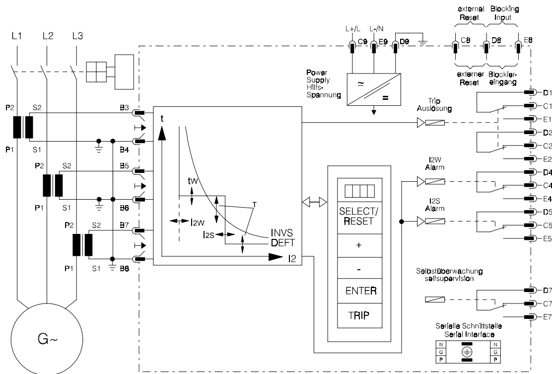
Fig. 3.1: Connection diagram
